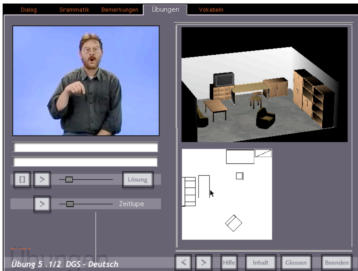
Fig. 7: Interactive exercise with context sensitive feedback (Metzger, Schulmeister, Zienert 2002)
