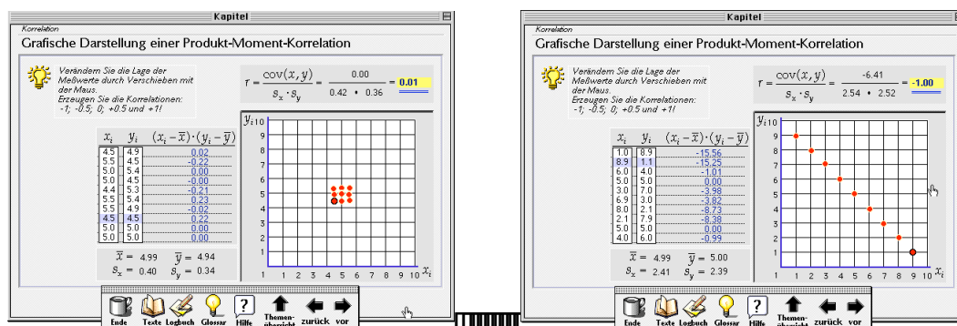
Fig. 5: Two scatterplots created by dragging the dots in the plot (Schulmeister/Jacobs 1992-1996)
