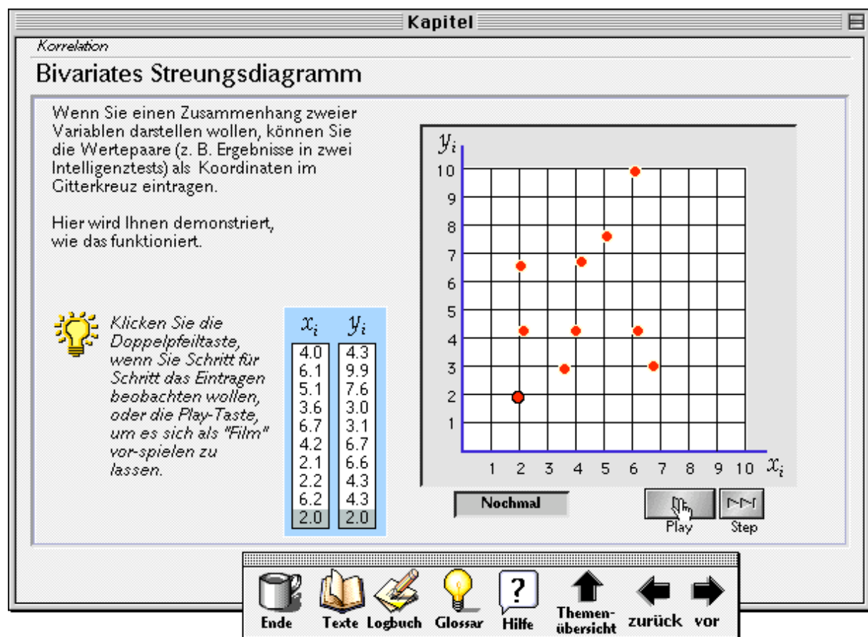
Fig. 8: Automatic program execution: Correlation diagram (Schulmeister/Jacobs 1992-1996)
